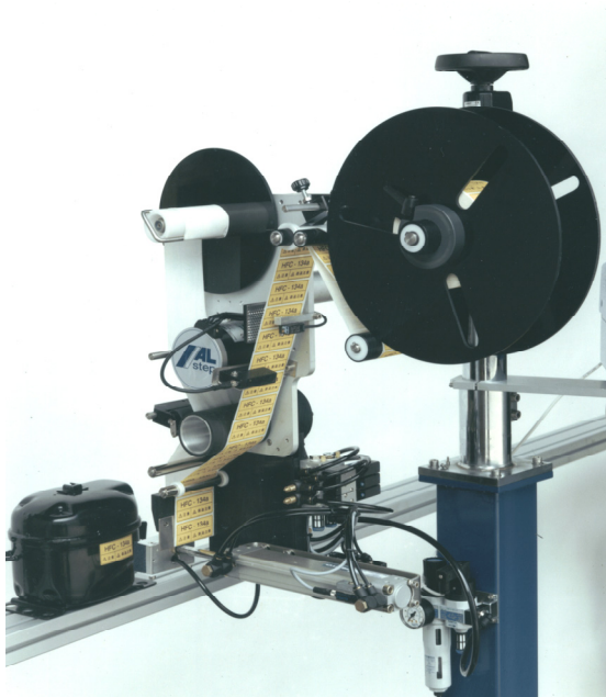
Standard machine with vacuum transfer assembly
